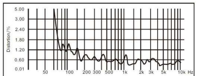
Distortion Characteristics (THD< 3% 1W, 1m, 100Hz-10kHz)
