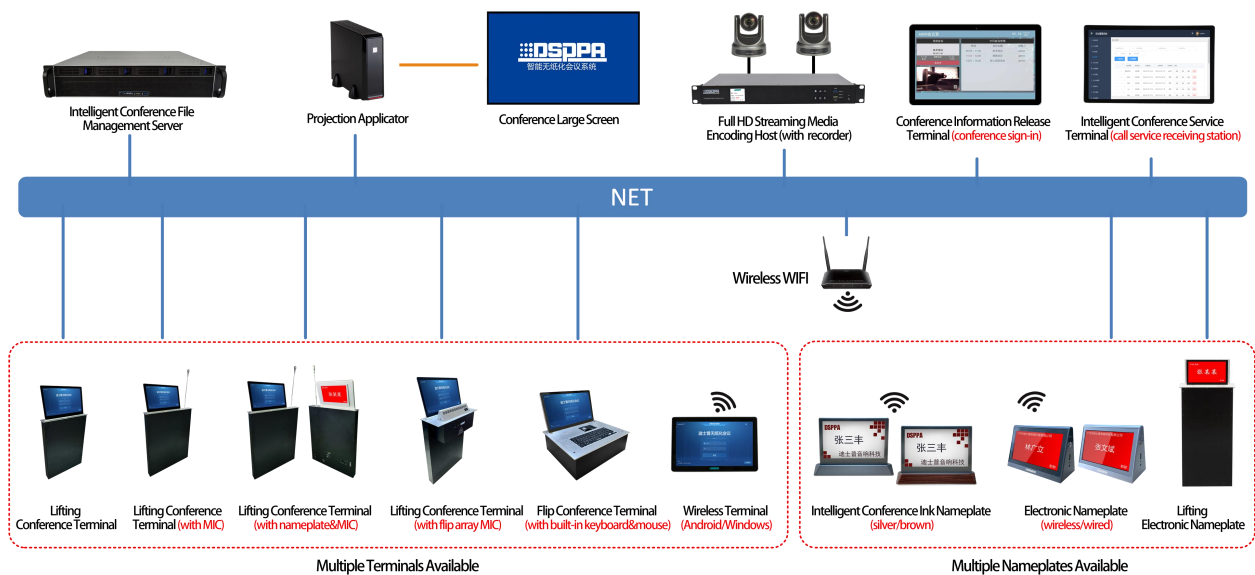
DSPPA Intelligent Paperless Conference System Topology
